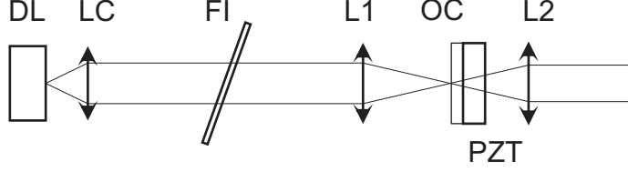
Fig. 1. Schematic of the external cavity laser using an interference filter (FI) for wavelength selection: (DL) laser diode, (LC) collimating lens, (OC) partially reflective out-coupler, (PZT) piezoelectric transducer actuating OC, (L1) lens forming a "cat's eye" with OC, (L2) lens providing a collimated output beam.
