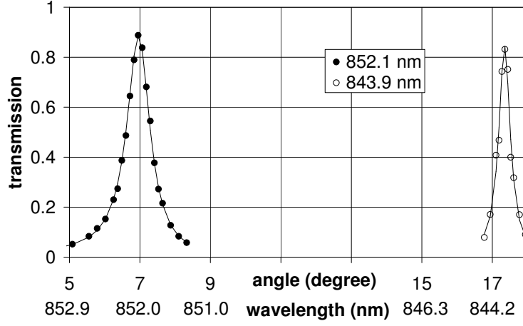
Fig. 2. Filter transmission of 852.1 nm light (●) and 843.9 nm light (○), as a function of the angle of incidence. The solid lines are Lorentzian fits to each peak.
